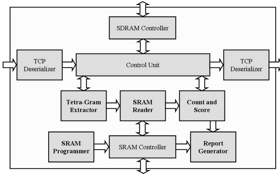
Fig. 2. Block diagram of HAIL's basic architecture
