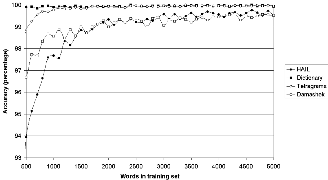
Fig. 3. Experimental results for language identification schemes using documents of one hundred words each.
